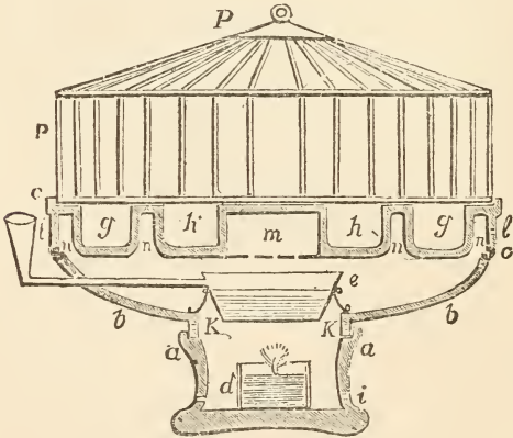
53. Lecoq's propagating-oven.
